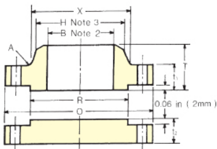
RAISED FACE
