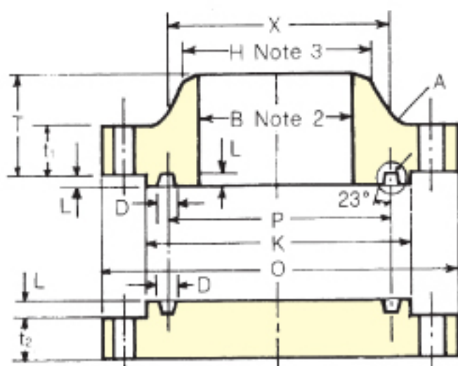
RING TYPE JOINT
